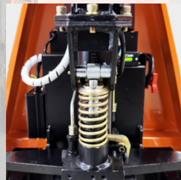
POWERED LIFT
